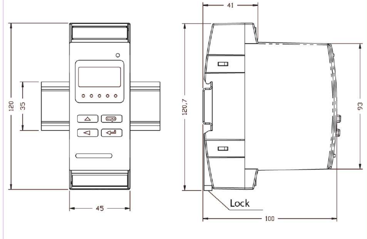
Fig. 2 Overall dimensions and mounting of the transducer.
